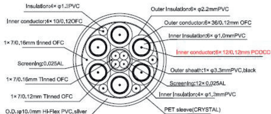
Structure Of Cable
